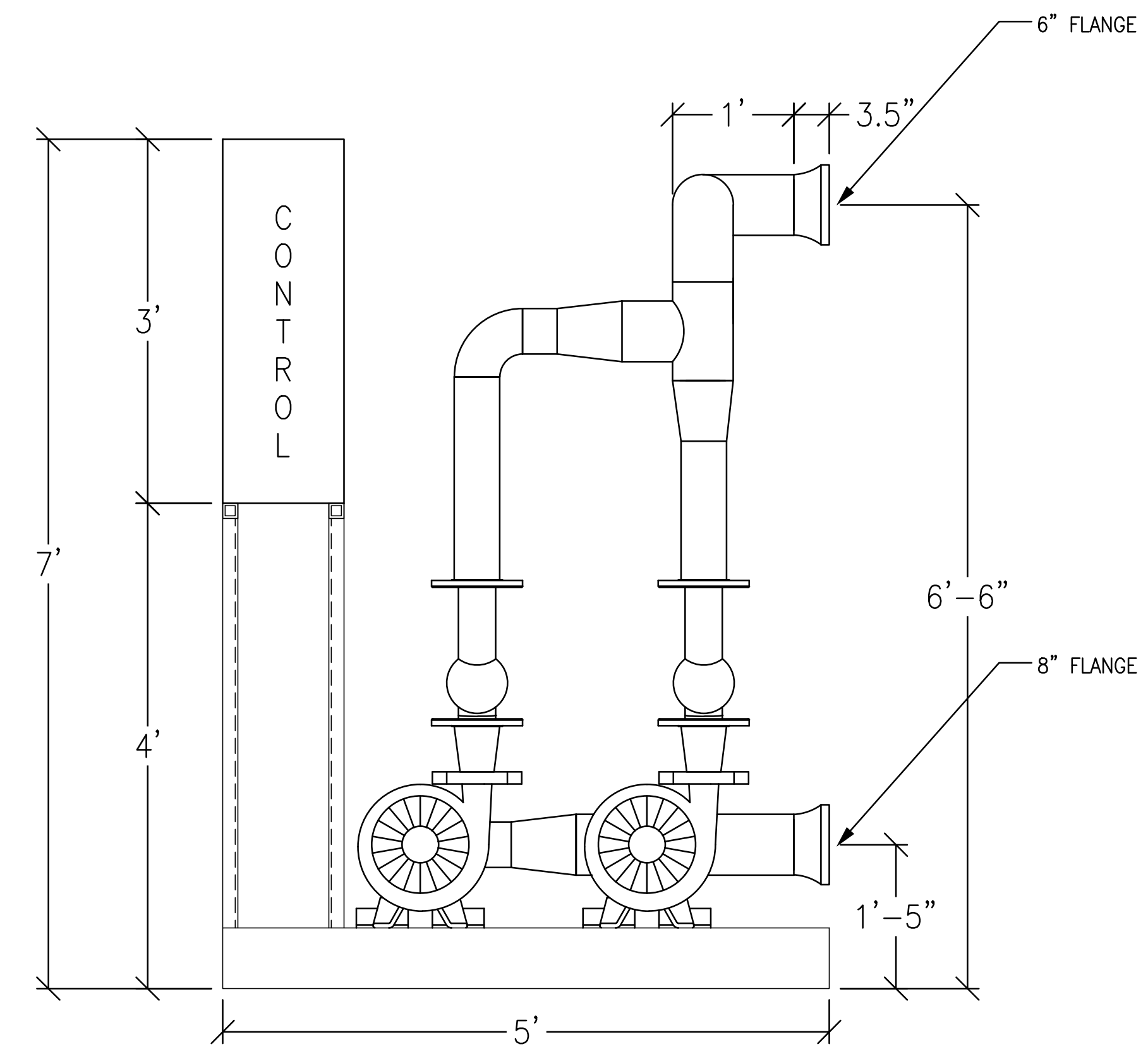
RIGHT VIEW WING - A,C
