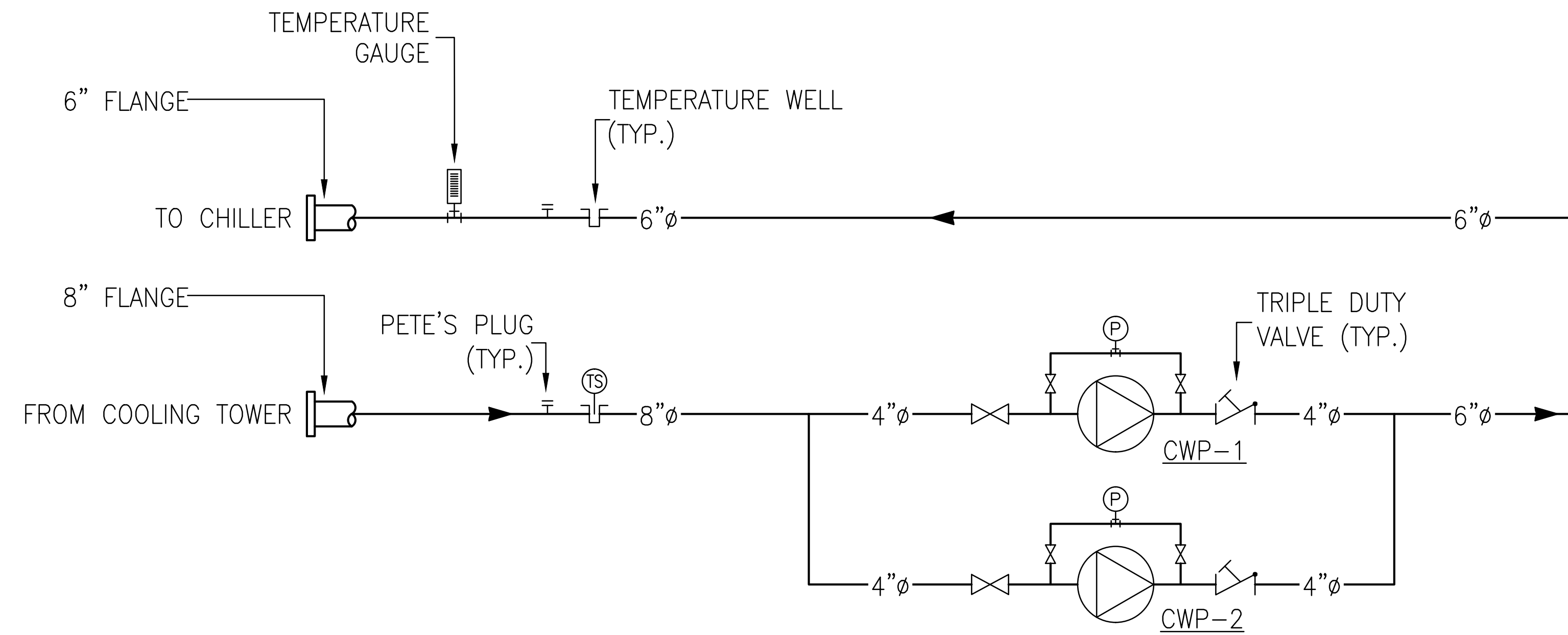
PIPING FLOW DIAGRAM (ALL WING OF BUILDING)
